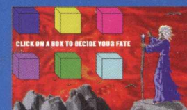
Wizard
