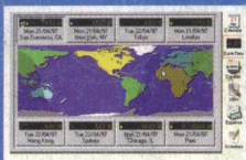
SideKick
